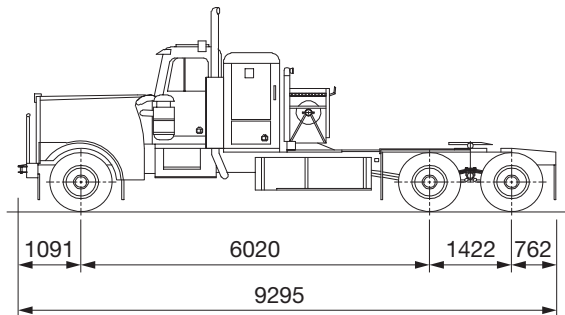
Kenworth W900
